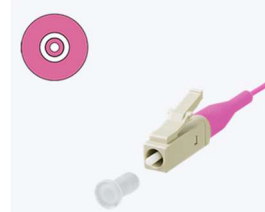
LC PC
